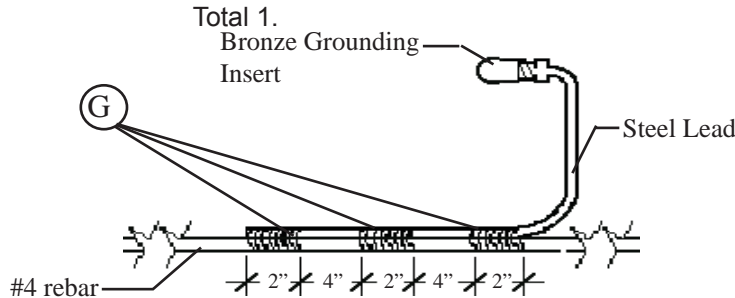
Enlarged View of Weld Detail
