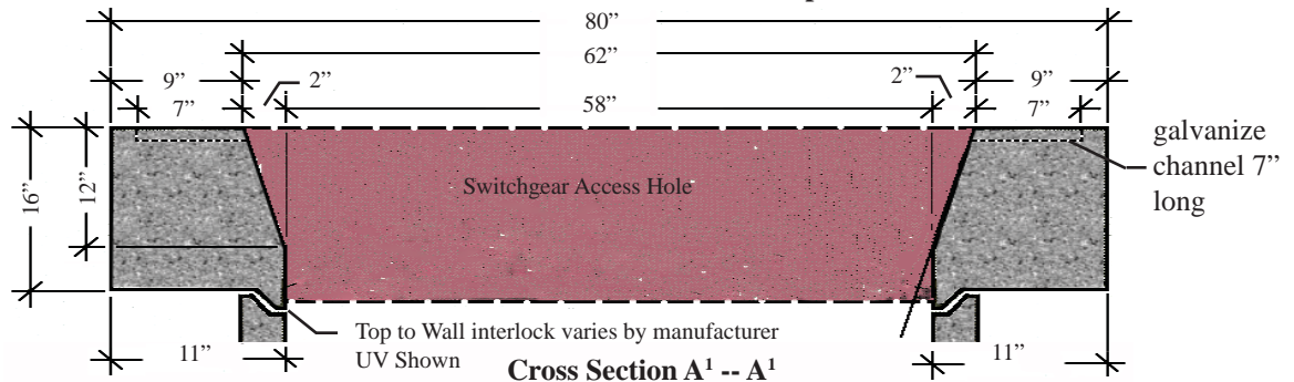
Cross Section Views of the Vault Top.
