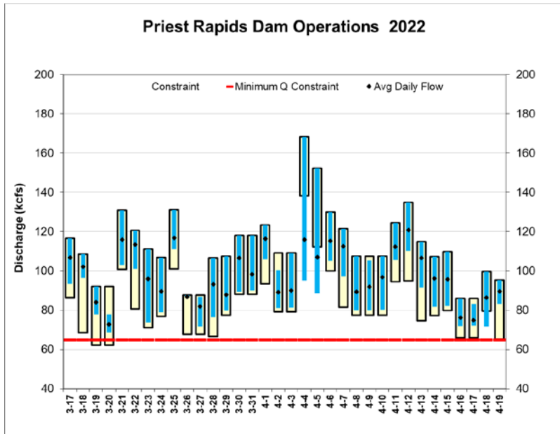
Figure 14 Mean, minimum, maximum hourly discharge and daily fluctuation from Priest Rapids Dam, March 17 – April 19, 2022.
