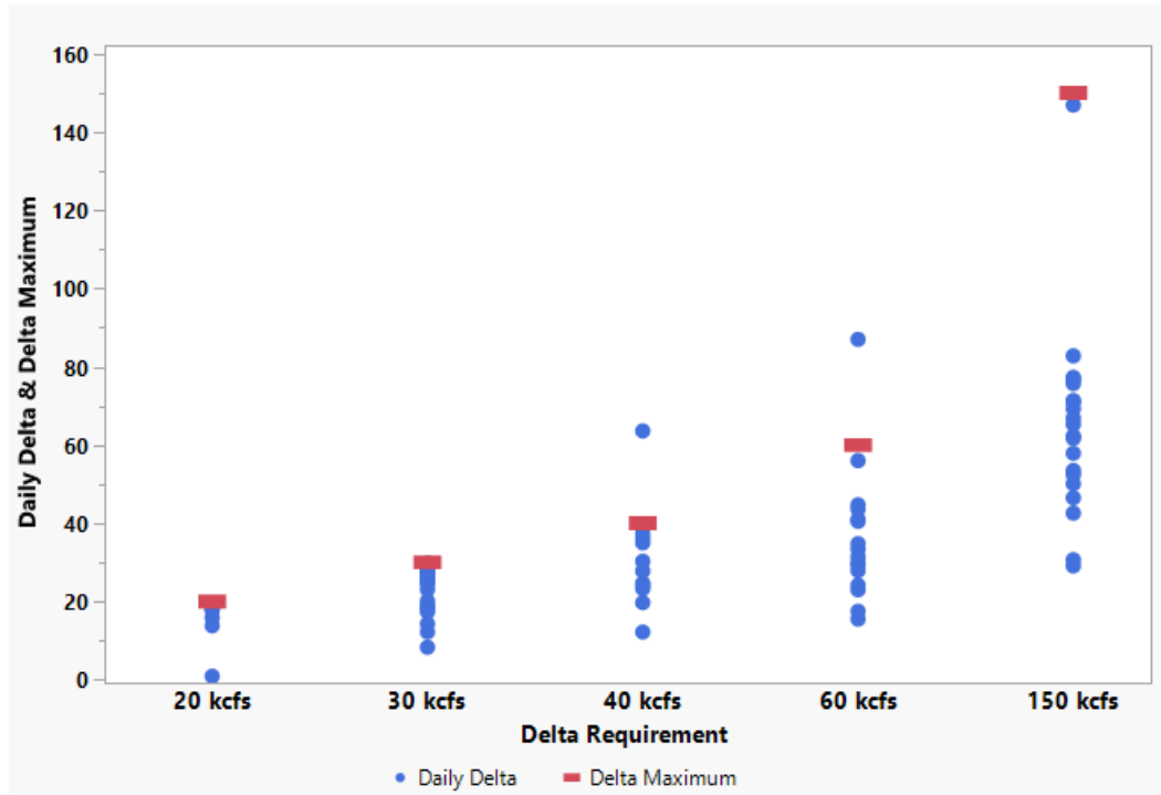
Figure 13 Summary of 2022 Priest Rapids Dam daily discharge deltas and delta maximum by constraint category.
