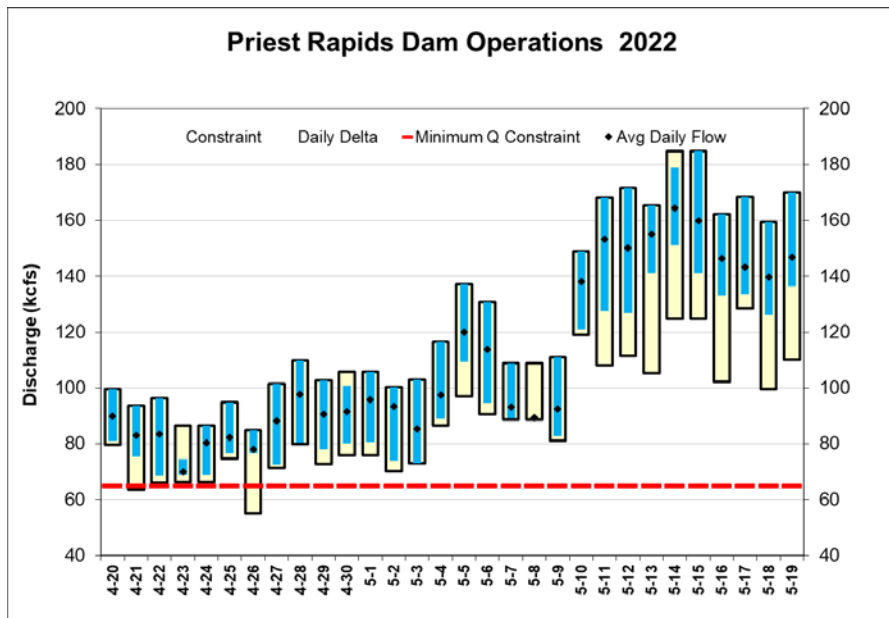
Figure 15 Mean, minimum, maximum hourly discharge and daily fluctuation from Priest Rapids Dam, April 20 – May 19, 2022.
