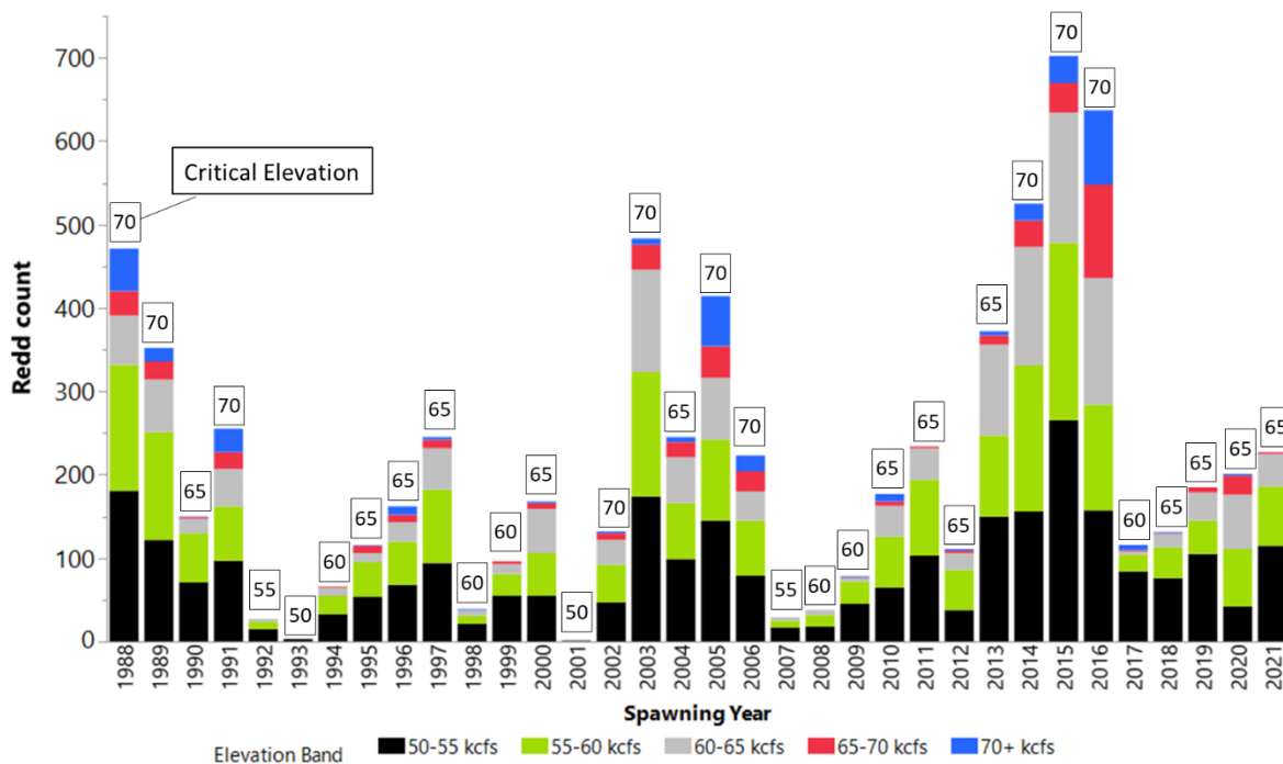
Figure 3 Final redd abundance and distribution from ground surveys on Vernita Bar, 1988-2021. Final redd count are not consistently conducted in the 36-50 kcfs zone and are not included in this figure. The Critical Elevation for each year is listed above the bars.
