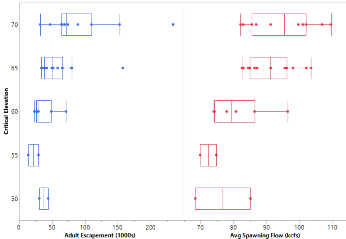
Figure 6 Relationship between Hanford Reach adult escapement and the Critical Elevation (left) and Priest Rapids Dam average discharge during peak spawning and Critical Elevation (right) (1988-2021).
